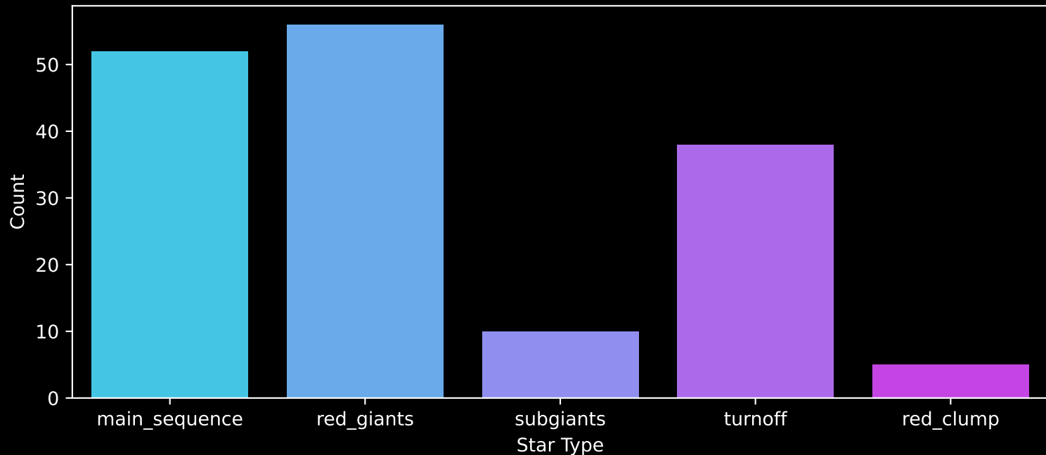
APOGEE DR17 Field: [065-29_MGA] Count plot of Star Type
