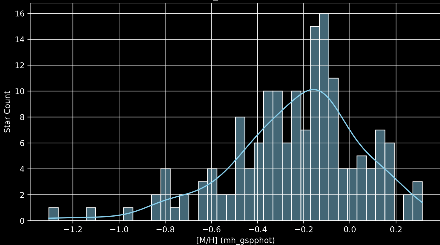
APOGEE DR17 Field: [065-29_MGA [M/H] (mh_gspphot) (n= 161)
