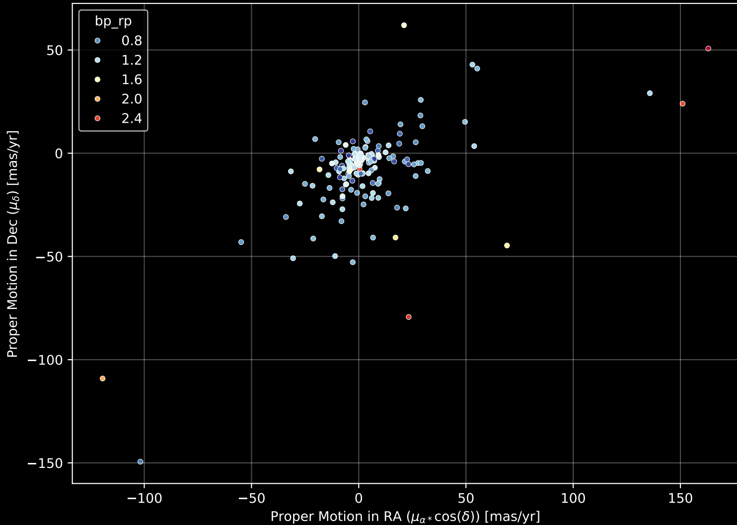
APOGEE DR17 Field: [065-29_MGA] Proper Motion Diagram (n= 161)
