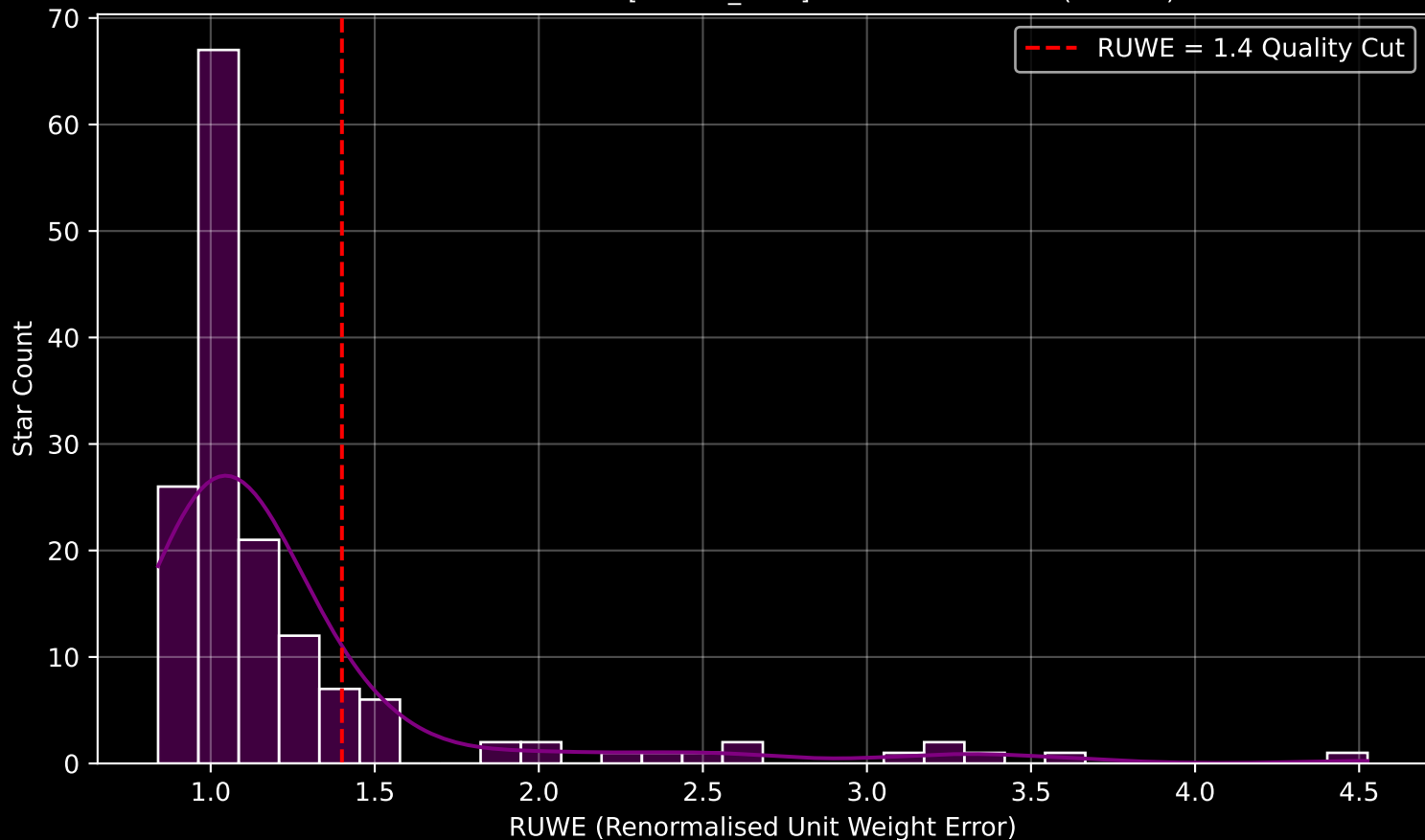
GAPOGEE DR17 Field [065-29_MGA] RUWE Distribution (n= 154)
