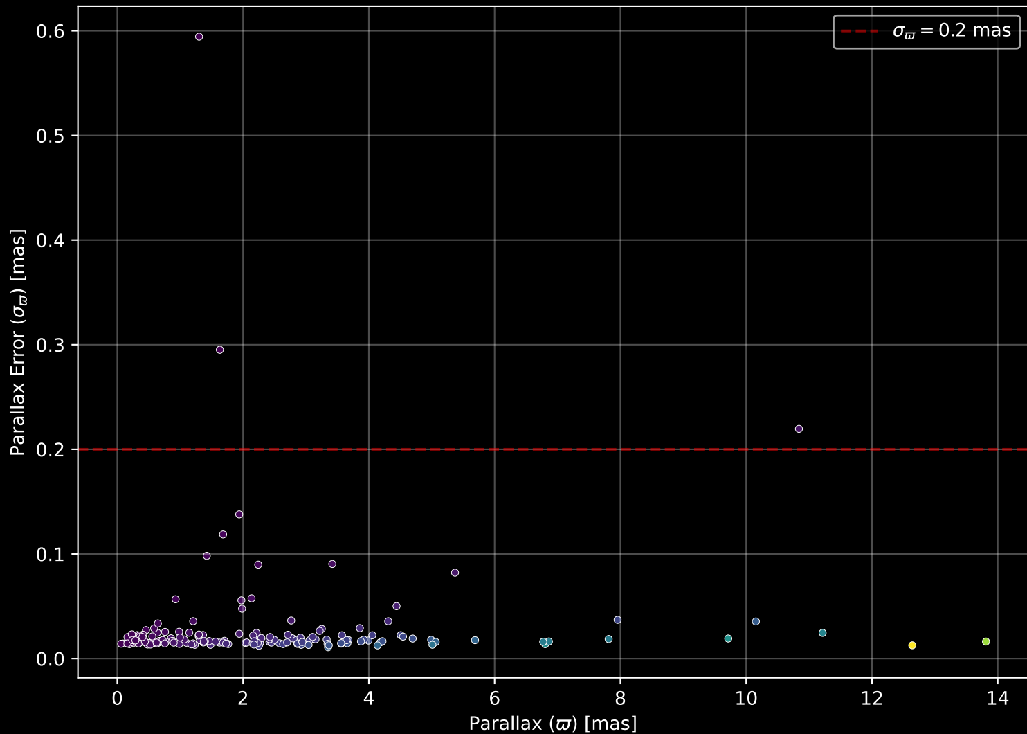
APOGEE DR17 Field: [065-29_MGA] Parallax Quality (n= 161)
